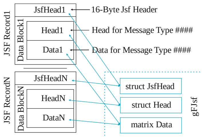
Figure 1.1 Jsf records structure
